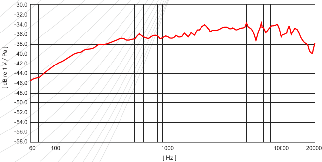
Frequency Response
