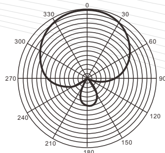
Polar Pattern
