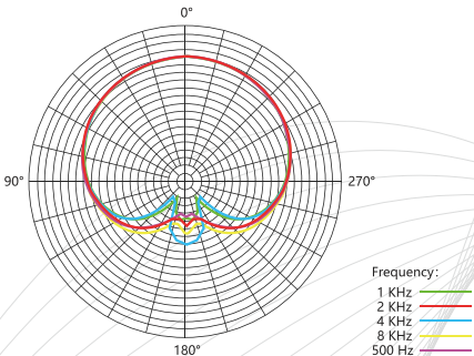
Polar Pattern
